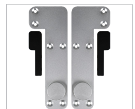
Small Brackets for Pattern Board on Standard Frame/IA800 Model# CSC050A-05 P/N: 50A-05
