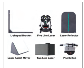
ADAS Accessory Kit (6 PCS)
