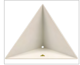
OE sized Corner Reflector Set (Mitsubishi) MODEL# CSC0802-12 P/N: 802-12
