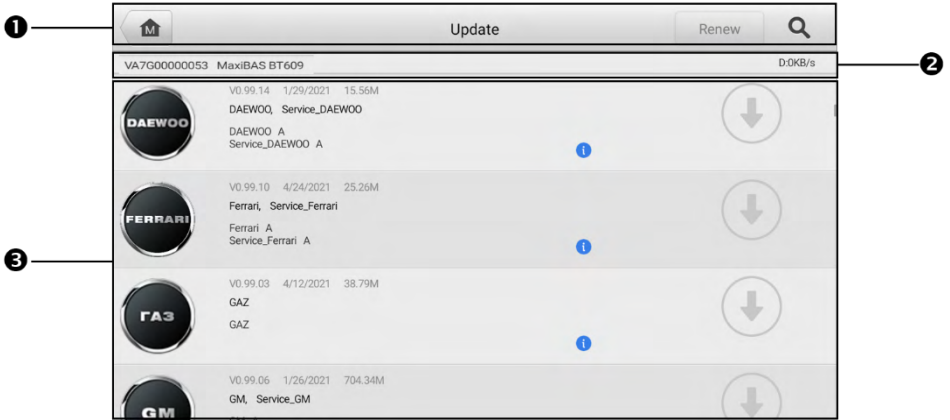
Figure 13-1 Update Screen
