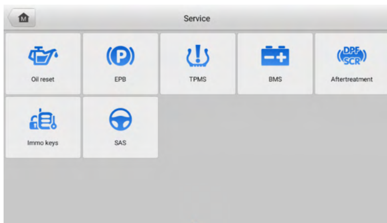
Figure 10-1 Service Menu
