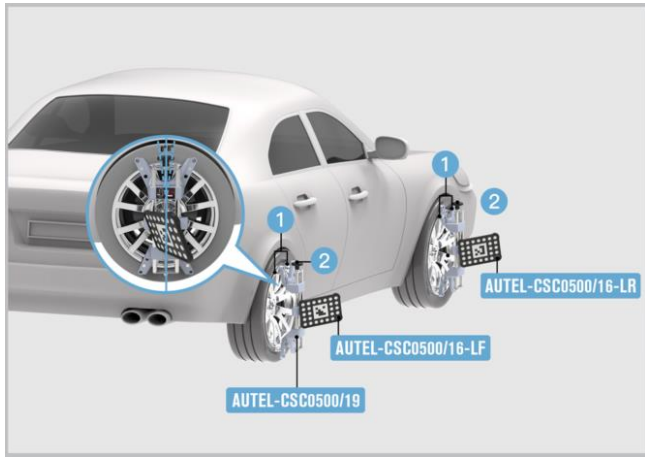
Figure 6-39 Install Wheel Clamps (Rim Clamps)
