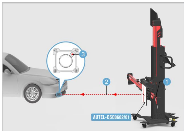
Figure 6-16 Align Laser with Mini Reflector
