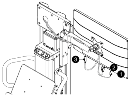
Figure 2-10 24" LCD Touchscreen Monitor
