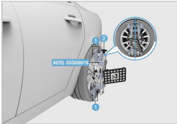
Figure 6-92 Install the Wheel Clamps (Rim Clamps)
