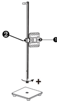
Figure 3-6 Alignment Aid AUTEL-CSC0500/08
