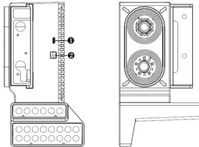
Figure 2-8 Left Camera Unit AUTEL-CSC0500/18
