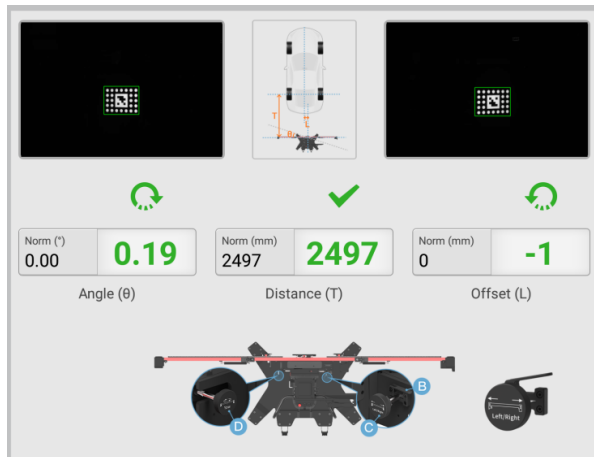
Figure 6-44 Position the Calibration Frame
