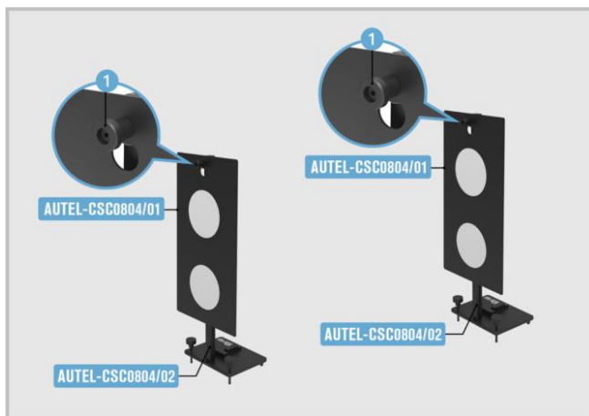
Figure 6-50 Mount the Target Board
