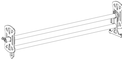
Figure 3-8 Calibration Bar — Suitable for Wheel Clamp (Rim Clamp)
