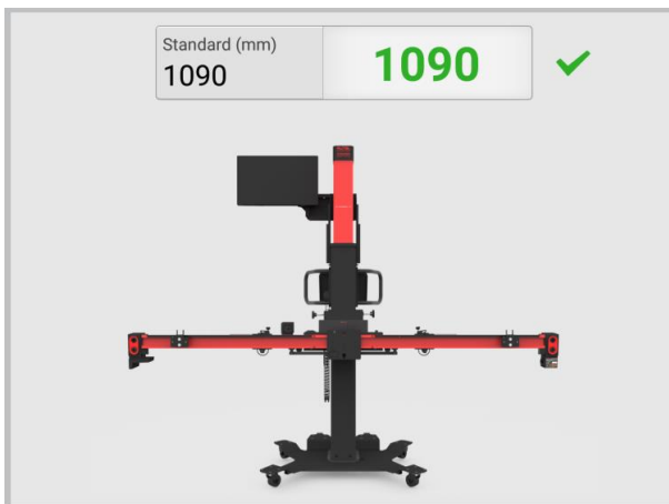
Figure 6-86 Adjust Standard Height
