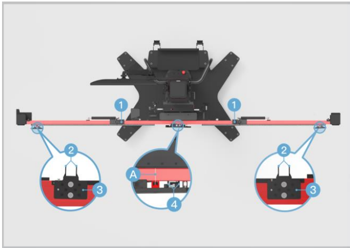
Figure 6-36 Position the Sliding Plate
