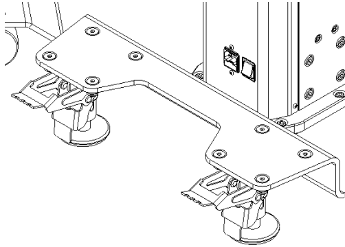
Figure 2-5 Two Footbrakes
