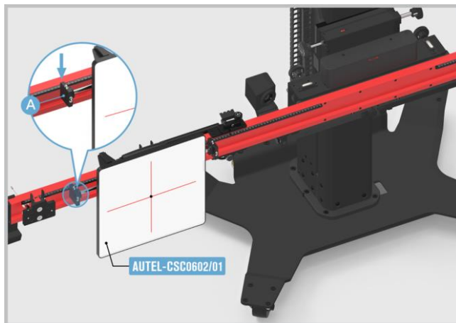
Figure 6-14 Adjust the Reflector 2
