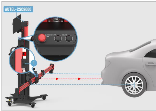
Figure 6-27 Center the Laser
