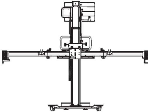
Figure 2-1 Calibration Frame AUTEL-CSC9000
