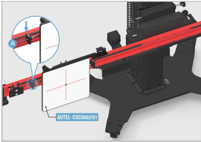
Figure 6-15 Adjust the Reflector 3
