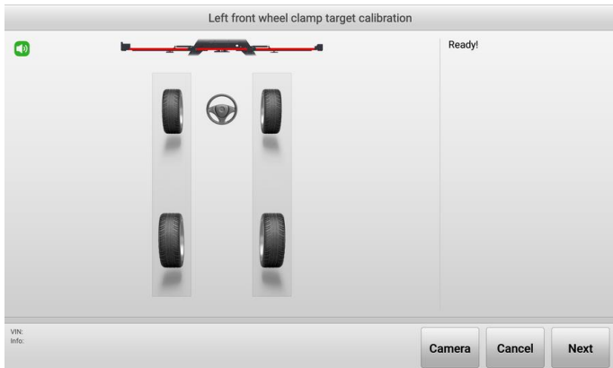
Figure 5-31 Start Calibration (Use Vehicle) 2
