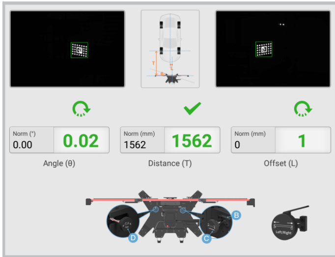
Figure 6-97 Position the Calibration Frame
