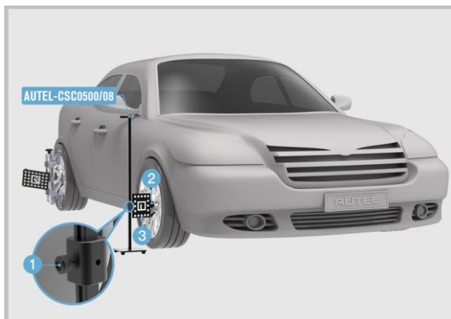
Figure 6-81 Adjust the Distance Measuring Target
