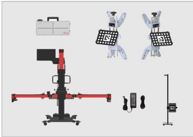
Figure 6-63 Required Calibration Tools
