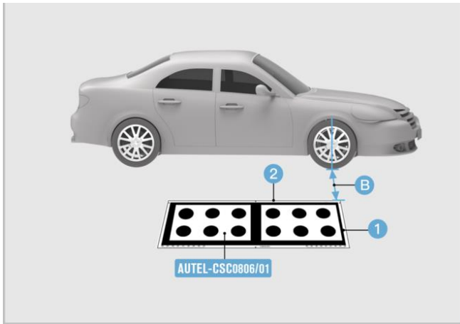
Figure 6-58 Calibrate Camera in Right Mirror 1
