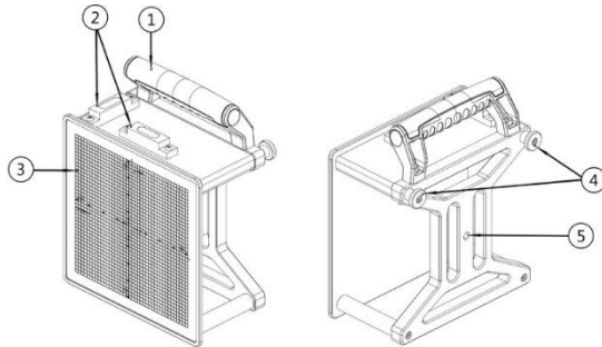
Figure 3-24 Radar Calibration Plate AUTEL-CSC0602/08
