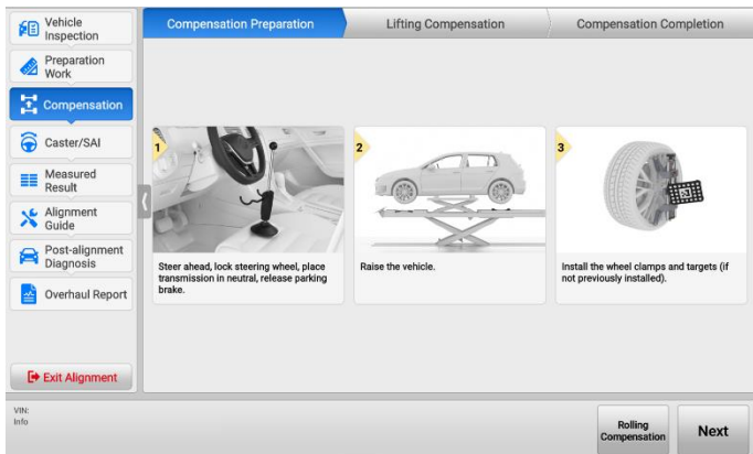
Figure 4-41 Lifting Compensation Preparation (Use Rim Clamp)
