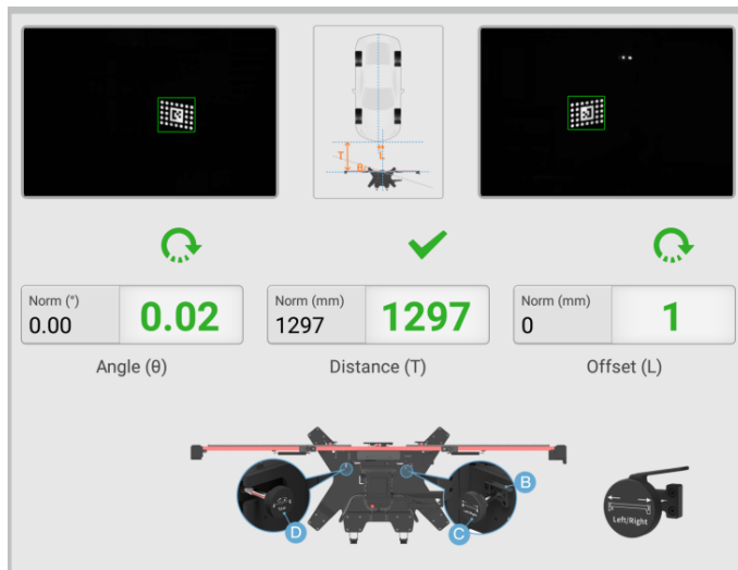
Figure 6-69 Adjust the Calibration Frame
