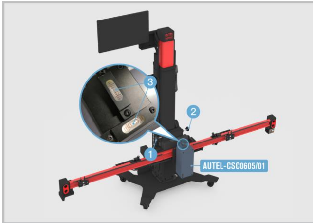
Figure 6-30 Center the Bubble Level of Radar Calibration Box
