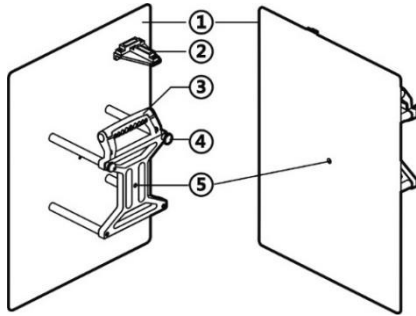
Figure 3-17 Radar Calibration Plate AUTEL-CSC0602/02
