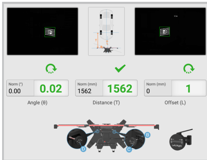
Figure 6-82 Adjust the Calibration Frame
