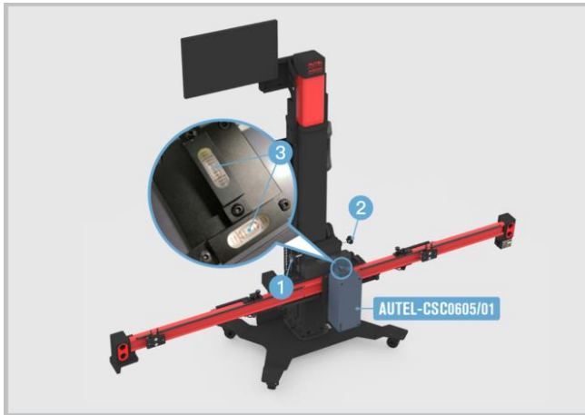
Figure 6-45 Center the Bubble Level of Radar Calibration Box
