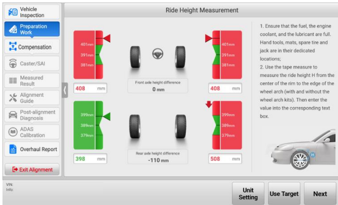
Figure 4-30 Measure Ride Height with Tape 1
