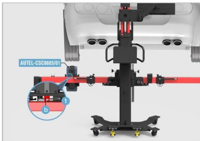
Figure 6-33 Move the Radar Calibration Box (Left)
