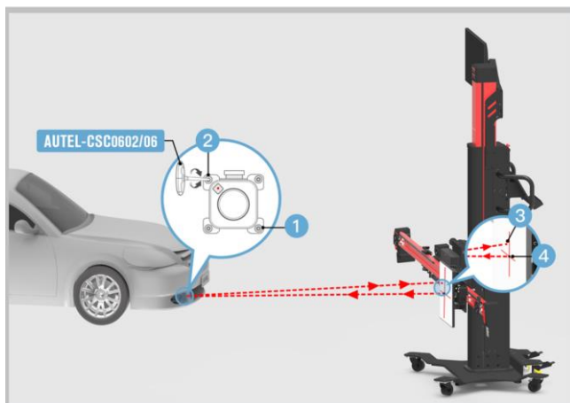
Figure 6-17 Align Reflected Laser with Origin Laser
