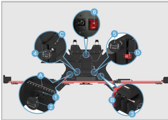
Figure 6-26 Align with Marked Lines
