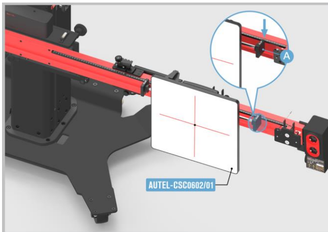
Figure 6-21 Adjust the Reflector 3
