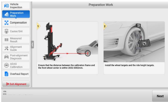
Figure 4-32 Install Ride Height Target
