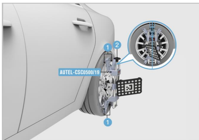
Figure 6-80 Install the Wheel Clamps (Rim Clamps)
