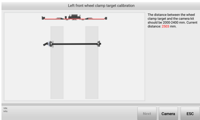
Figure 5-22 Start Calibration (Use Calibration Bar) 1
