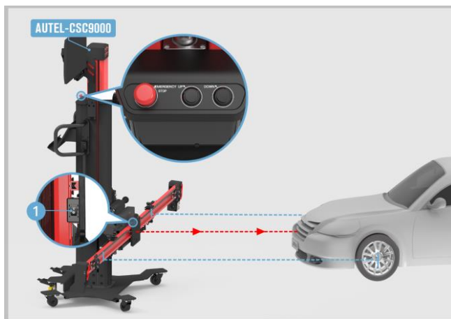
Figure 6-79 Center the Laser
