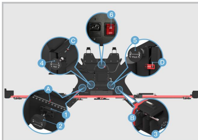
Figure 6-65 Align with Marked Lines
