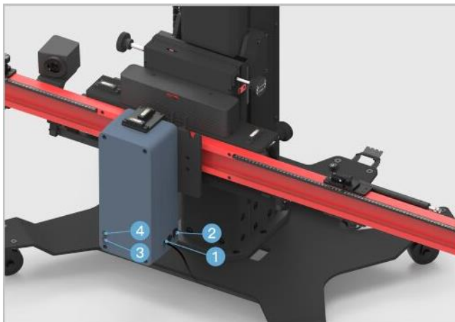
Figure 6-31 Connect Power
