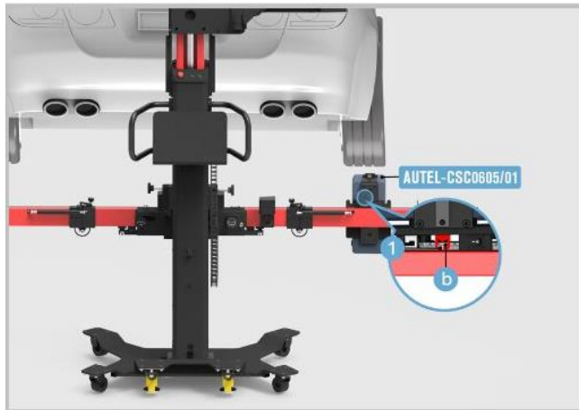
Figure 6-34 Move the Radar Calibration Box (Right)
