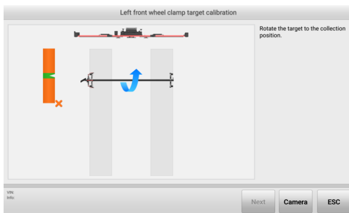
Figure 5-24 Start Calibration (Use Calibration Bar) 3
