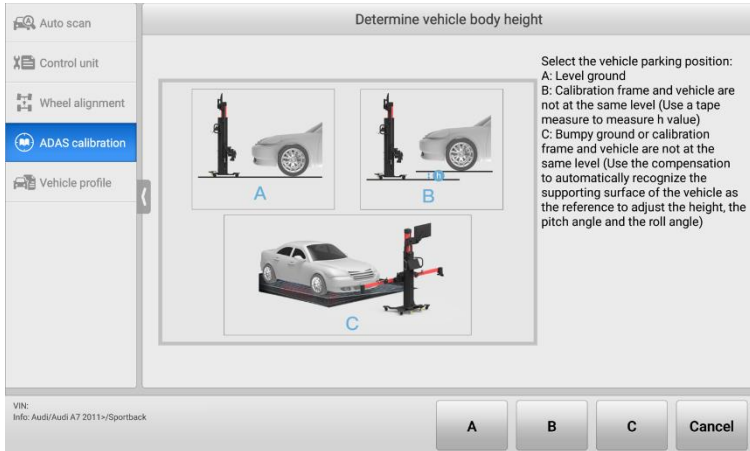
Figure 6-74 Select Vehicle Parking Position
