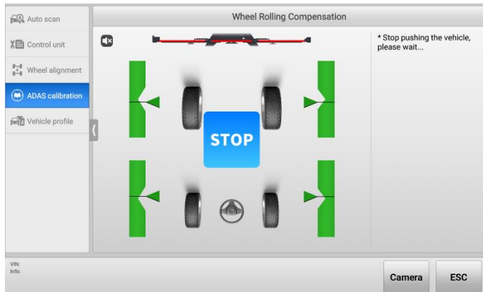
Figure 6-96 Wheel Rolling Compensation 4
