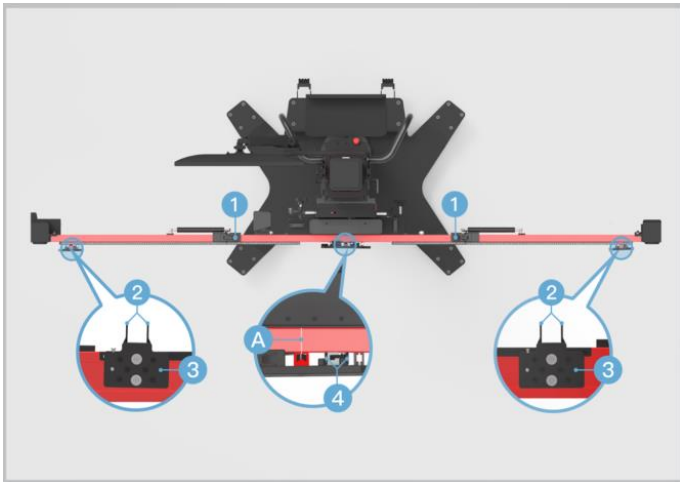
Figure 6-64 Position the Sliding Plate
