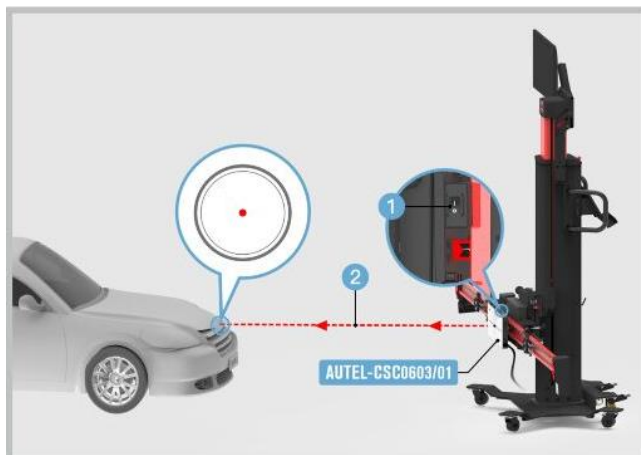
Figure 6-72 Center the Laser
