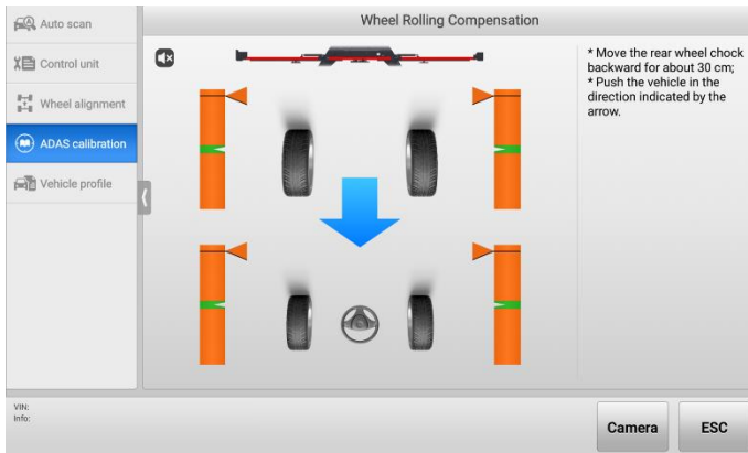
Figure 6-40 Wheel Rolling Compensation 1
