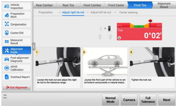
Figure 4-59 Adjust Right Tie Rod
