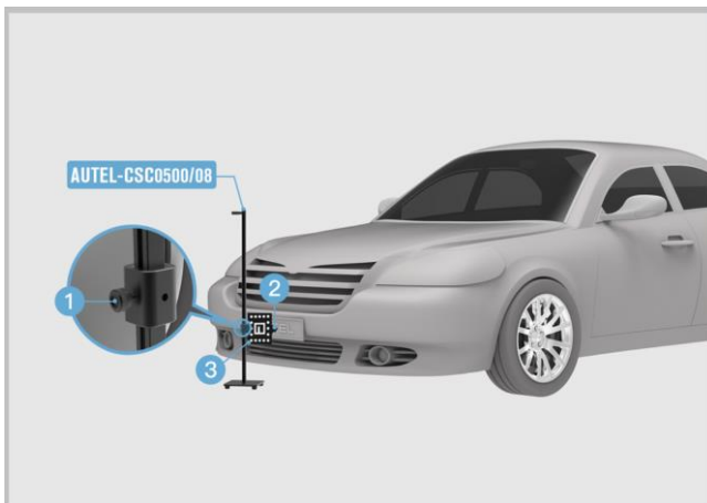
Figure 6-6 Adjust the Distance Measuring Target
