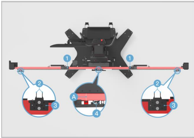
Figure 6-77 Position the Sliding Plate
