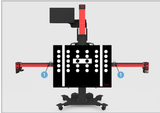
Figure 6-100 Fix the Target Board
