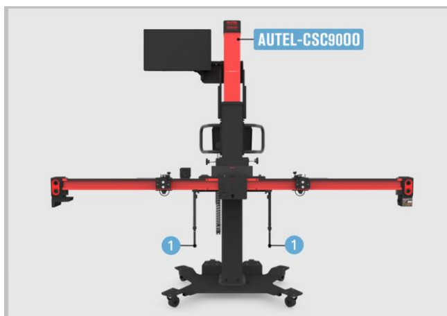
Figure 6-99 Extend Target Board Holder
