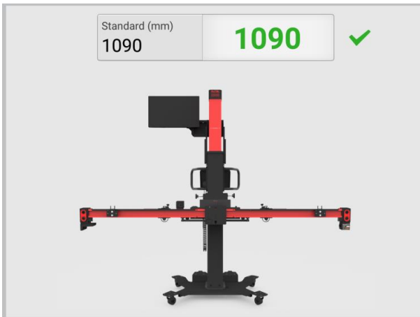
Figure 6-101 Adjust Standard Height
