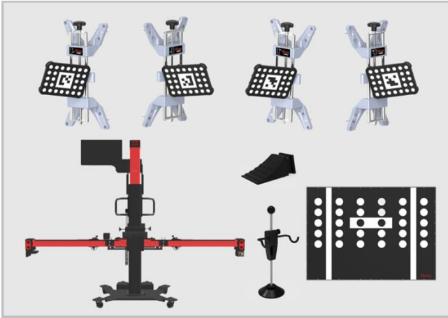
Figure 6-88 Required Calibration Tools
