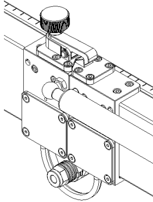
Figure 2-3 Folding Mechanism
