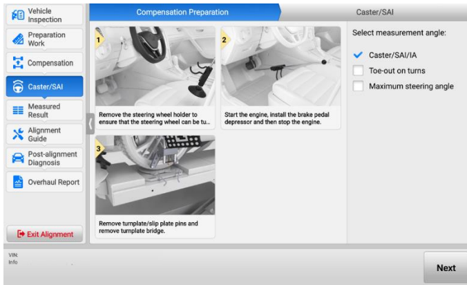
Figure 4-47 Caster/SAI/IA Measurement
