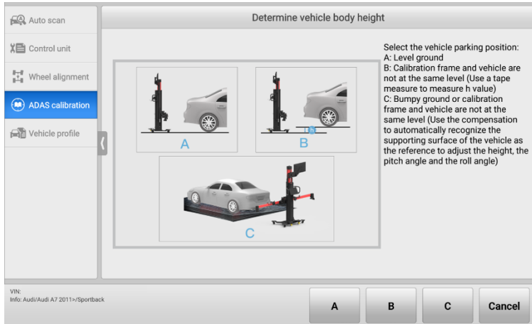
Figure 6-22 Select Vehicle Parking Position
