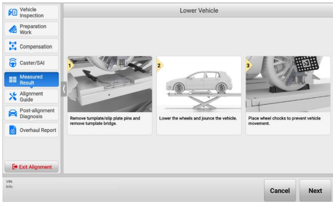
Figure 4-53 Lower Vehicle
