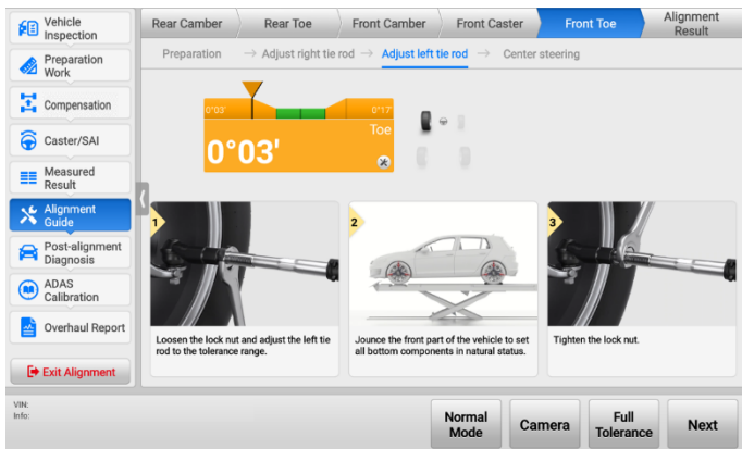
Figure 4-60 Adjust Left Tie Rod
