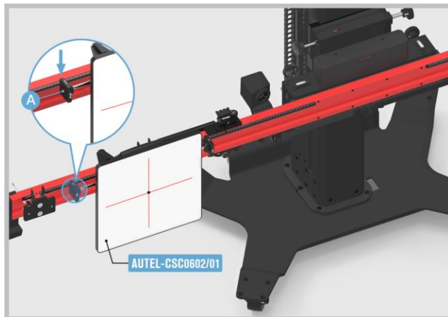
Figure 6-13 Adjust the Reflector 1
