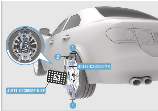
Figure 6-28 Install the Wheel Clamps (Rim Clamps)
