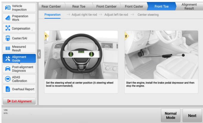
Figure 4-58 Front Toe Adjustment Preparation
