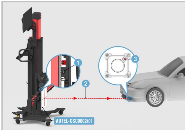
Figure 6-10 Align Laser with Mini Reflector
