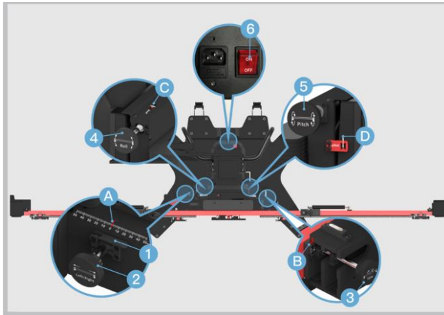
Figure 6-78 Align with Marked Lines
