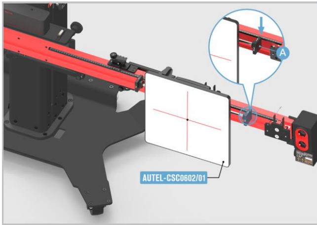
Figure 6-19 Adjust the Reflector 1
