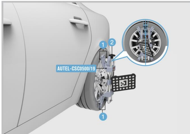
Figure 6-5 Install the Wheel Clamps (Rim Clamps)
