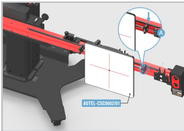
Figure 6-20 Adjust the Reflector 2
