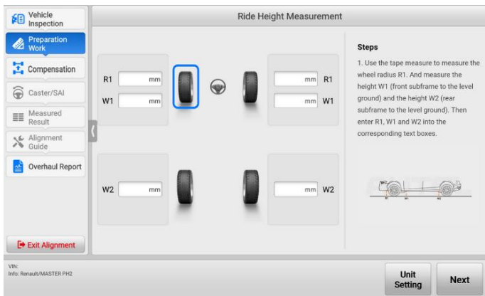
Figure 4-31 Measure Ride Height with Tape 2
