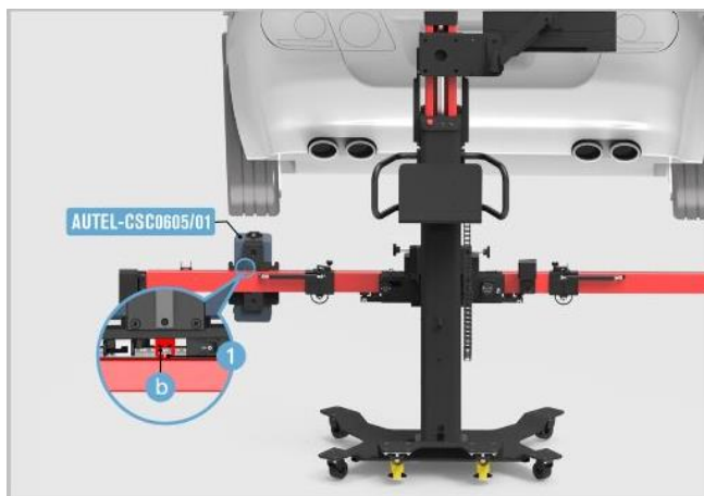
Figure 6-48 Move the Radar Calibration Box (Left)
