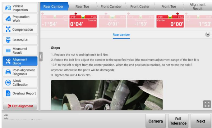
Figure 4-55 Parameters Adjustment Procedures Screen 1
