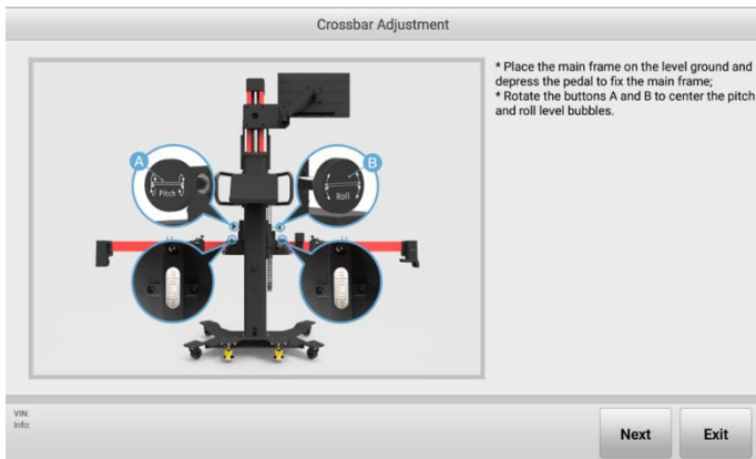
Figure 5-8 Crossbar Adjustment 1
