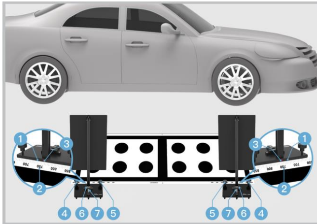
Figure 6-59 Calibrate Camera in Right Mirror 2
