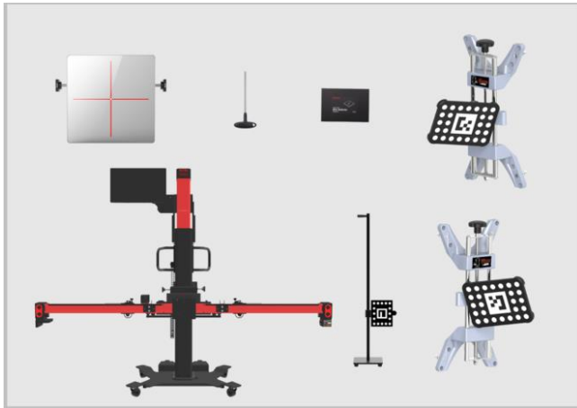
Figure 6-1 Required Calibration Tools
