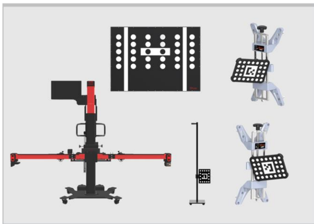
Figure 6-76 Required Calibration Tools (When Selecting A or B)
