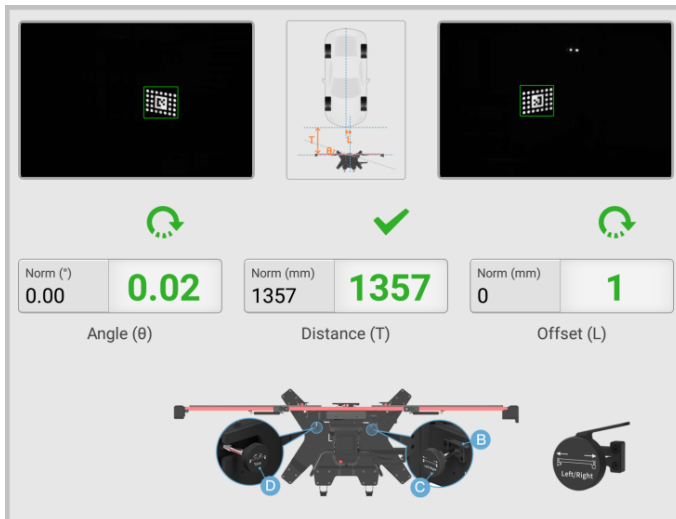
Figure 6-7 Adjust the Calibration Frame
