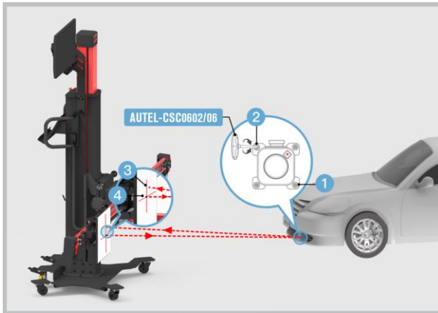
Figure 6-11 Align Reflector Laser with Origin Laser
