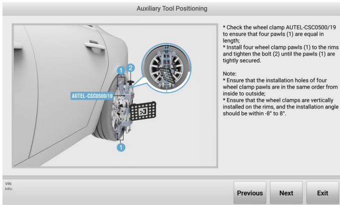
Figure 5-54 Auxiliary Tool Positioning 4
