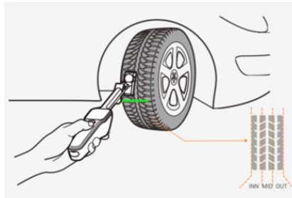
Figure 4-18 MaxiTPMS TBE Device (not included) and Use Diagram
