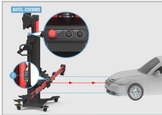
Figure 6-4 Center the Laser
