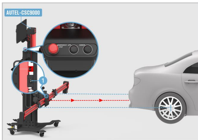
Figure 6-38 Center the Laser
