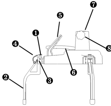
Figure 3-2 Wheel Clamp (Tire Clamp) AUTEL-CSC0500/17
