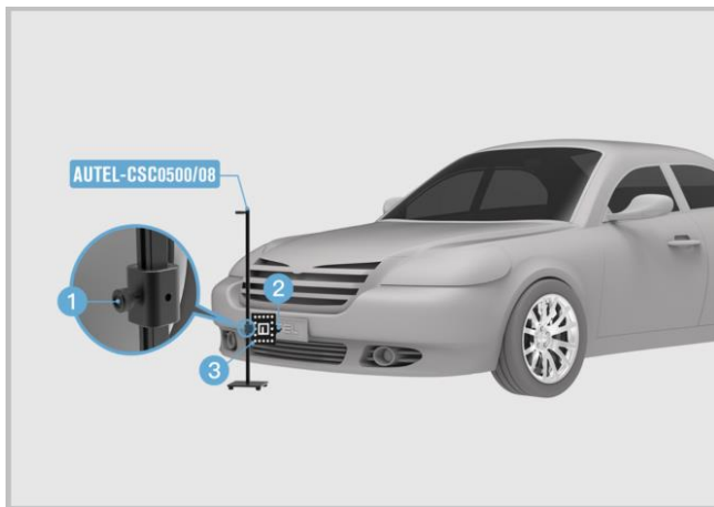
Figure 6-68 Adjust the Distance Measuring Target
