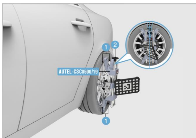
Figure 6-67 Install the Wheel Clamps (Rim Clamps)
