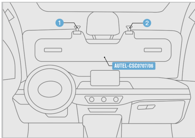
Figure 6-60 Place HUD Calibration Board
