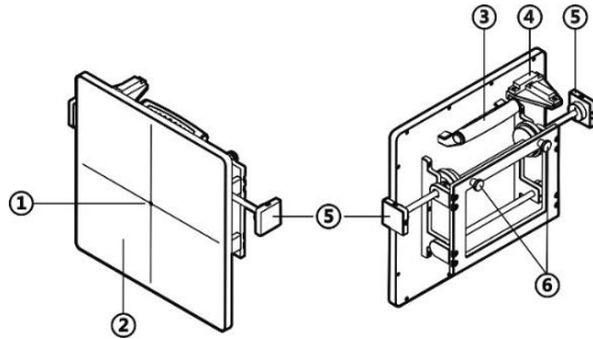
Figure 3-14 Reflector AUTEL-CSC0602/01
