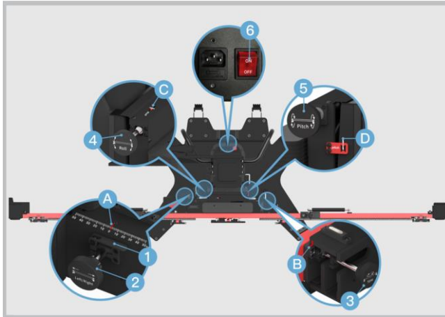
Figure 6-37 Align with Marked Lines
