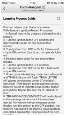
Figure 4-27 Sample Stationary Relearn Screen 2
